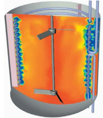
The temperature on a slice through the reactor after about 11 minutes of cooling
