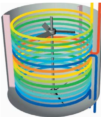
Two sets of cooling coils are used in the reactor to keep the temperature controlled
